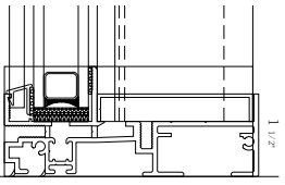
Regular Sill
