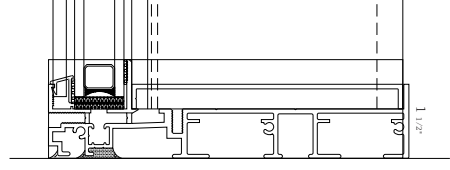
Heavy Sill
