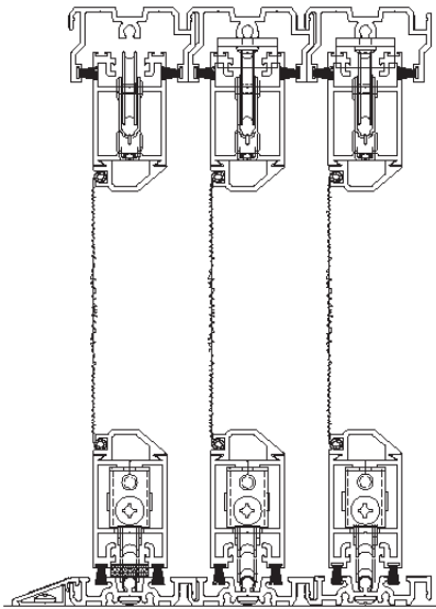
Head and Sill
