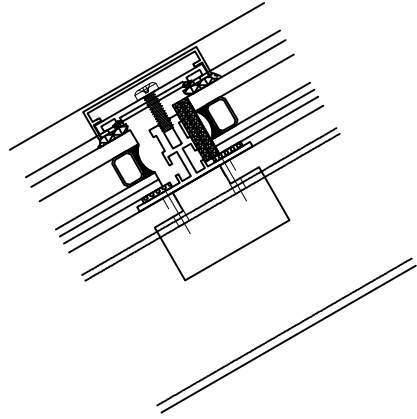
SECTION VIEW TYPICAL 1" BOXED MUNTIN DETAIL W/ REGULAR BAR SLOPED RAFTER
