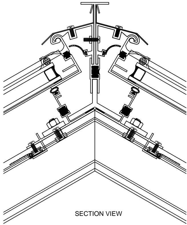
SECTION VIEW RIDGE VENT HEAD DETAIL W/ REGULAR BAR SLOPED RAFTER
