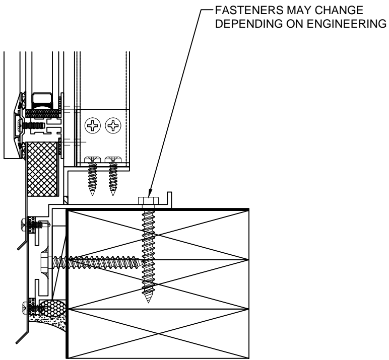
SECTION VIEW TYPICAL SILL DETAIL AT ENDWALL BAR GABLE H5201
